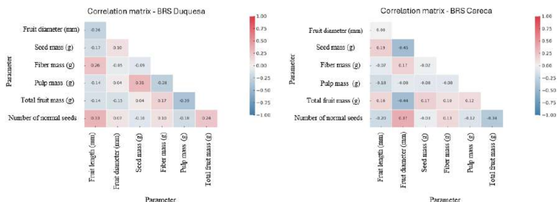
Figure 1 - Correlation matrix of the main biometric parameters of BRs Duquesa and BRS Careca.
